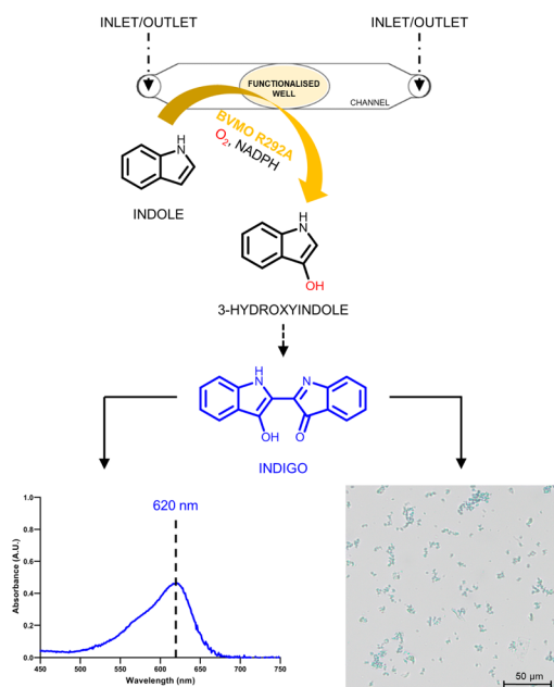
Fig. 2 Indigo formation and detection. Ar-BVMO R292A is immobilized on the bottom glass surface of a small well placed in the middle of a channel structure. The immobilized enzyme catalyses the hydroxylation of indole in presence of molecular oxygen and NADPH. The final product, indigo, is a coloured compound that can be detected spectrophotometrically (absorbance peak at 620 nm) or microscopically (formation of small blue particles).
