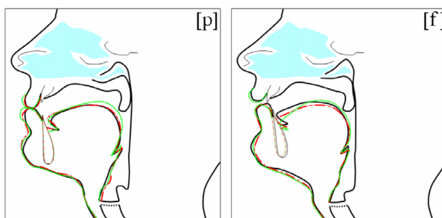
Figure 7. Outline hand-tracings of the articulatory configurations detected in the bilabial and labio-dental places for the realisations of /p/ (left) and /f/ (right) in /VCV/ utterances with V=/a/ (plain line), V=/i/ (dashed line) V=/u/ (dotted line).
