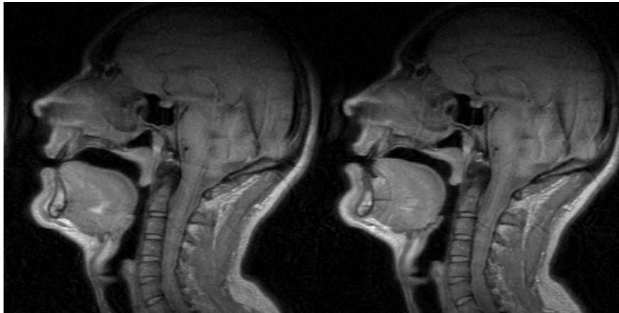
Figure 3. MRI scans for C in an utterance of / h aC:#Ca/ with C articulated in a alveodental place for a lamino-alveolar realisation of /s/ (left) and in a (post)alveolar place for a labialised realisation of /ʃ/ (right).
