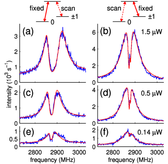
FIG. 3 (color online). Measured and fitted fluorescence intensity vs modulation frequency, using the middle excited state of an N-V with excited-state level spacings (see Fig. 1) a = 0.31 GHz and b = 0.94 GHz. (a,c,e): laser fixed on m_s = 0 transition; (b,d,f): laser fixed on m_s = \pm 1 transition. Excitation powers: (a,b): 1.5 \mu\text{W} ; (c,d): 0.5 \mu\text{W} ; (e,f): 0.14 \mu\text{W} .
