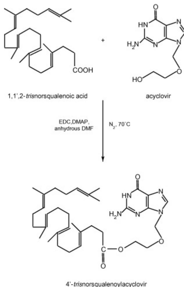
Fig. 1. - Reaction scheme for the synthesis of 4'-trisinorsqualenylacyclovir.
