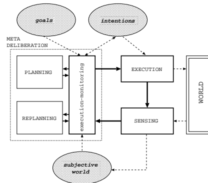
Fig. 1. The structure of the agent architecture. Dashed lines represent data flow, solid lines represent control flow.
