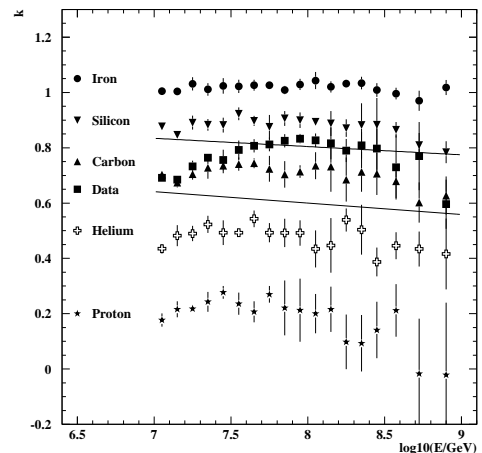
Figure 8: Evolution of the k parameter as a function of the reconstructed energy for experimental data compared with pure primary spectra for the entire angular range 0-40^{\circ} .
