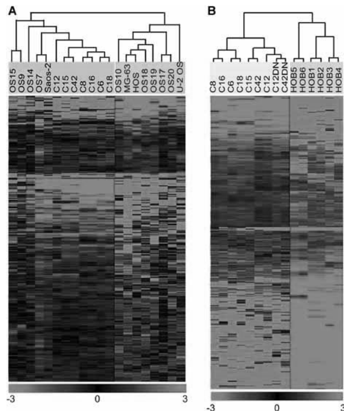
Figure 1 Microarray data-clustering of the human MET-OS clones, compared with the osteosarcoma cell lines (A) and to the parental bone-derived cells (B). Bioinformatic analysis of the indicated cell samples was performed using the Multi-Experiment Viewer 4.1 application. The cluster analysis organized the samples according to the similarities and dissimilarities of their expression profiles, placing the samples with similar expression profiles together as neighboring columns in the clustergram ( atop ). (A) Comparison of the MET-OS clones and the osteosarcoma cell lines (listed atop ). The hierarchical clustering of 300 genes differentially expressed >3 \log_2 -fold shows grouping of the MET-OS clones (C6, C8, C12, C15, C16, C18, C42) with a group of osteosarcoma cell lines (Saos-2, OS7, OS15, OS9, and OS14, green). These sample groups are both clearly distinct from the second group of osteosarcoma cell lines (red). (B) Comparison of the MET-OS clones and the parental bone-derived cells (HOB 1–6, indicated according to their original preparation numbers). The hierarchical clustering of the 311 genes differentially expressed >3 \log_2 -fold shows that the MET-OS clones (blue) are clearly separated from the HOBs (pink). The DN-MET-OS clone variants (C12DN, C42DN) clustered with the MET-OS clones from which they were derived (GSE28256; GSE28252; http://www.ncbi.nlm.nih.gov/geo/ ).
