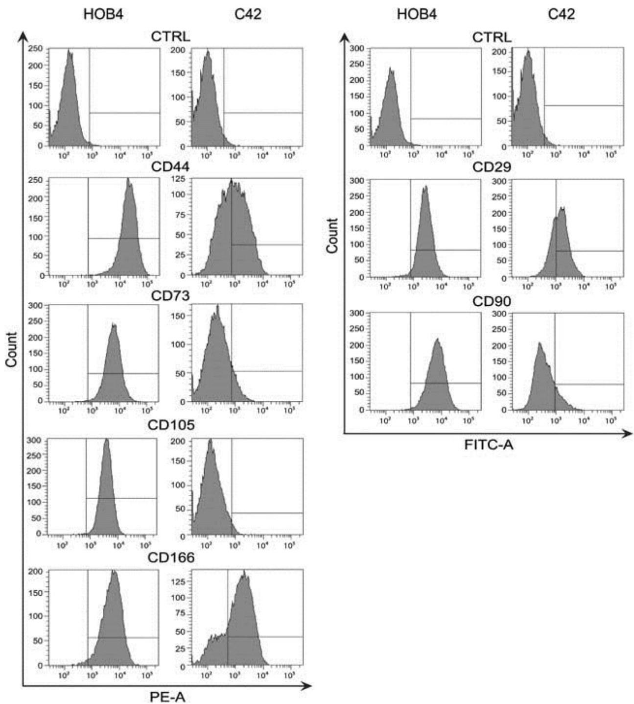
Figure 2 Differential expression of phenotypic MSC markers in the MET-OS clones versus the parental bone-derived cells. FACS analysis shows the different expressions of the MSC markers (as indicated) in the MET-OS clone (C42) and in the parental bone-derived (HOB4) cells.
