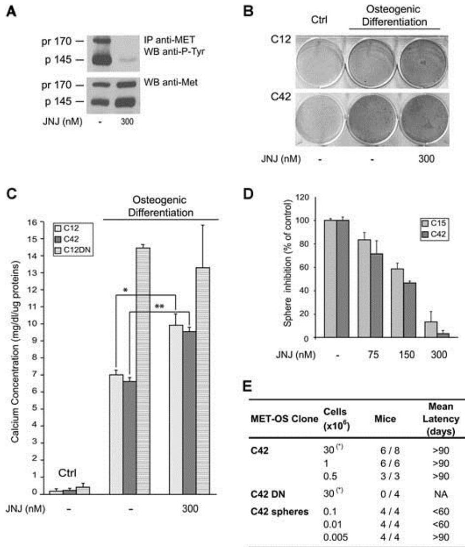
Figure 5 The self-renewal ability and differentiation potential of the MET-OS clones depend on MET activation. (A) The MET kinase small-molecule inhibitor JNJ-38877605 abrogated MET activation in the MET-OS clone C42, where MET was constitutively activated because of its overexpression. 26 JNJ-38877605 (B–C) and the expression of a dominant-negative form of the MET receptor (C12DN) (C) allowed cell progression towards osteoblastic differentiation, as demonstrated by osteomatrix production (B) and quantified as calcium released by the cells (C), after 14 days of osteogenic induction. (D) JNJ-38877605 inhibited sphere formation in the MET-OS clones (C15 and C42) seeded at low density under serum-free conditions. (E) Injection of the MET-OS clones into immune-compromised mice resulted in xenograft growth: NOD/SCID (C42 and C42 DN) and NOD-SCID IL2rg -/- (C42 spheres) have been injected. The number of mice with tumors out of the mice injected is shown. (*) data already shown in 26.
