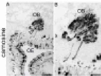
Figure 2 Carnosine staining in the olfactory pit during development (E15 mouse). A) At this stage, carnosine besides strongly labelling cell bodies and axonal projections of mature ORNs, is associated to a population of cells (arrowhead) migrating from the olfactory placode to the presumptive olfactory bulb (OB, olfactory bulb; OE, olfactory epithelium). Scale bar: 55 \mu\text{m} . B) Higher magnification detail of the previous image showing a carnosine-positive migrating cell entering the rostral tip of the OB within a bulk of carnosine-positive ORNs axons. Scale bar: 20 \mu\text{m} .
