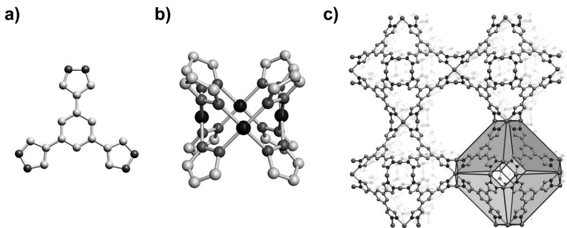
Figure 1: 5 a) Triply deprotonated form of the H 3 BTP linker used in the synthesis of the M 3 (BTP) 2 series of MOFs; b) depiction of the secondary building unit (SBU) of Ni 3 (BTP) 2 , showing the square-planar Ni 4 cluster bridged by eight exo-bidentate pyrazolate groups; c) Structure of Ni 3 (BTP) 2 with one of the sodalite cages highlighted. Black, dark grey, and light grey spheres represent Ni 2+ cations, nitrogen atoms and carbon atoms respectively. Hydrogen atoms are omitted for clarity.
