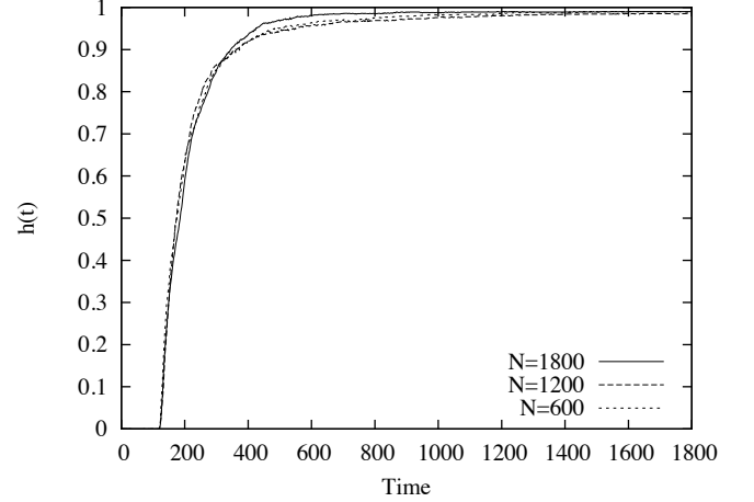
Fig. 10: h(t) as a function of time for T = 2.5s and w = 10s for different system sizes.
