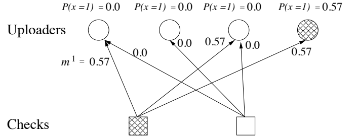
Fig. 8: Node pass computation example
