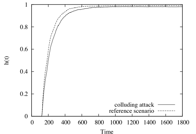
Fig. 5: h(t) as a function of time in case of a colluding attack.
