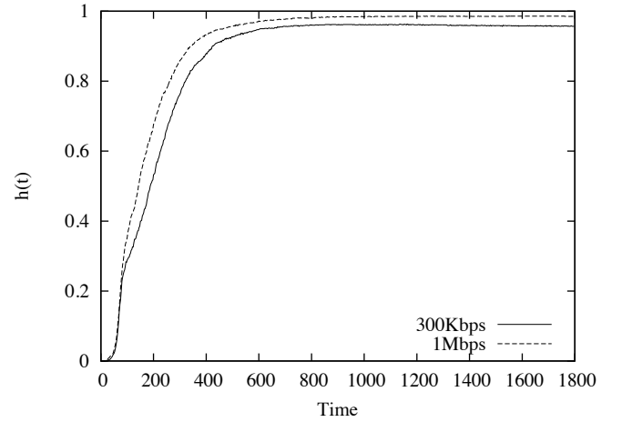
Fig. 14: h(t) as a function of time for churning, always lying, stealth malicious peers.
