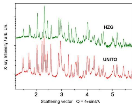
Fig. 1 e PXRD pattern of the partially hydrogenated 2\text{NaH} \cdot \text{D MgB}_2 . HZG [ PXRD pattern collected at the Helmholtz-Zentrum Geesthacht; UNITO [ PXRD pattern collected at the University of Turin.
