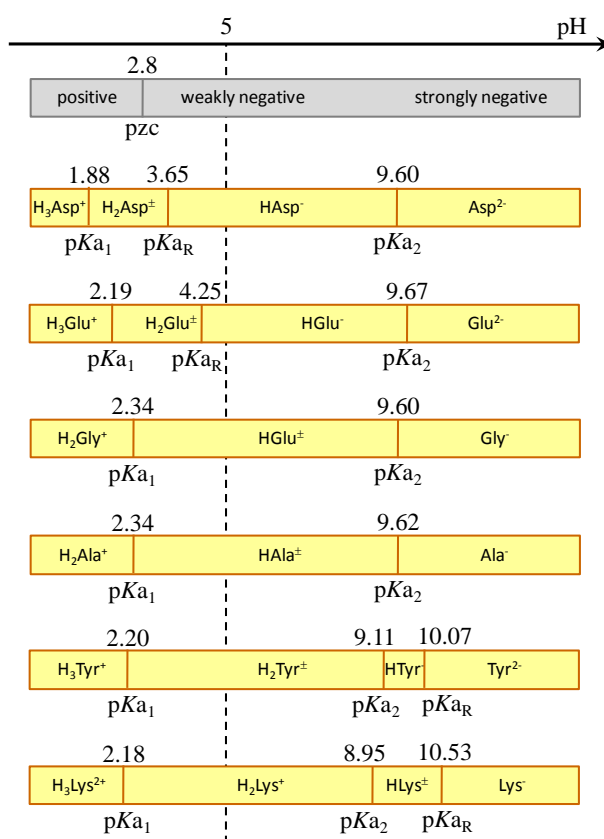
Figure 78. Theoretical acid-base speciation of the \alpha -quartz and the AA tested in Ref. 105 as a function of pH. pK a1 , pK a2 and pK aR refer to pK a values for backbone COOH, NH 3 + and side chain R groups, respectively.
