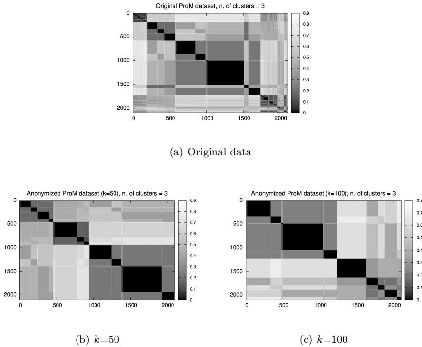
Fig. 9 Clustering results on ProM dataset (3 clusters)
