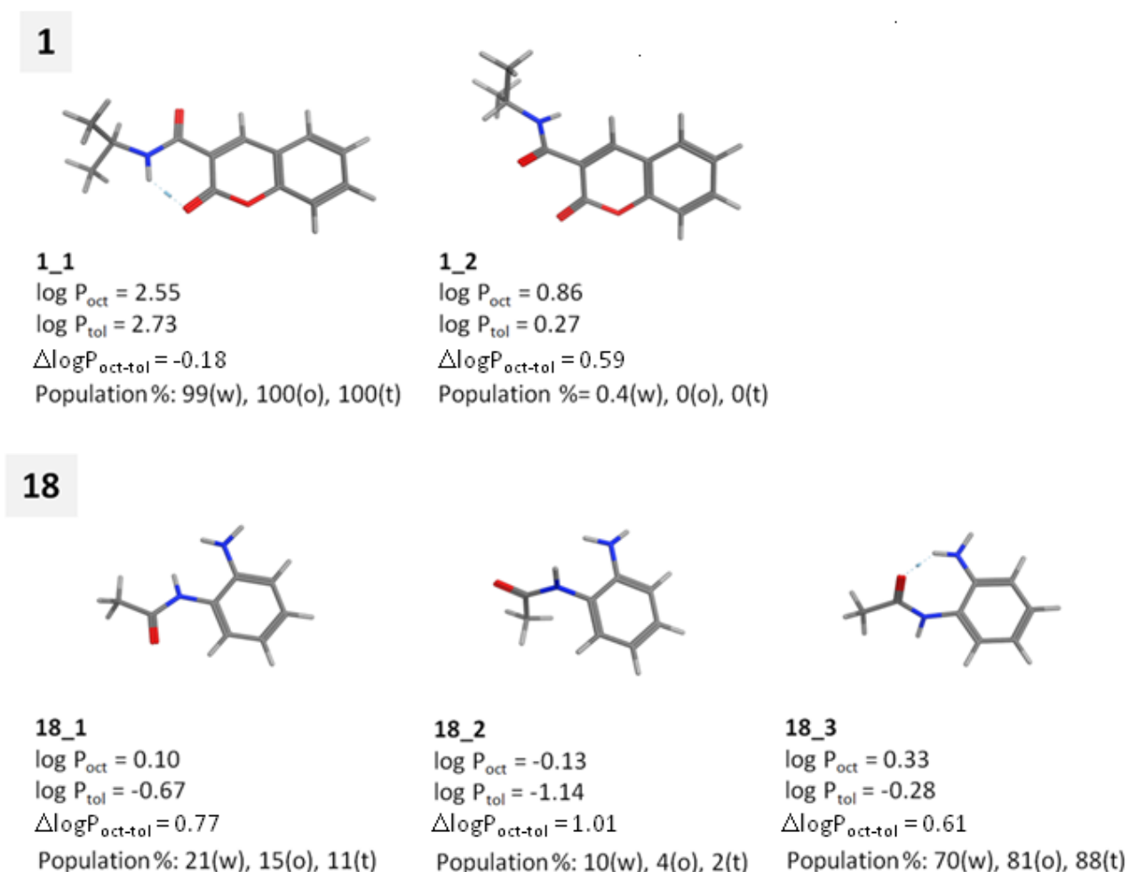
Figure 3. Examples of COSMO-RS results for conformations of compounds 1 (Category I, high propensity to form IMHB) and 18 (Category II, low propensity to form IMHB). The relative conformer populations in water (w), wet octanol (o) and toluene (t) are shown. For each conformer logP oct and logP tol were calculated ignoring all other conformations.
