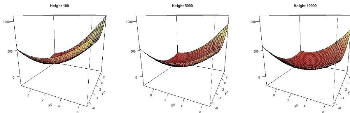
Fig. 9 \delta_0(x^0, y^0, h) for three different values of height
