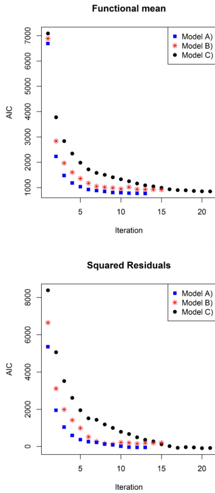
Fig. 5 AIC for f and AIC for g by iteration
