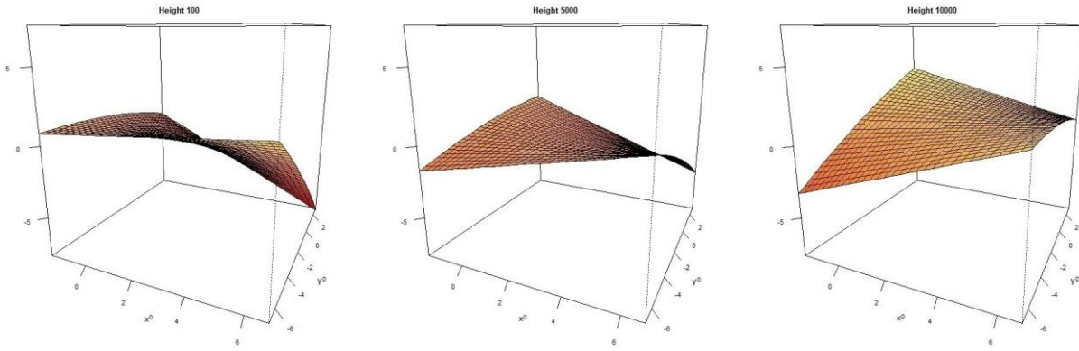
Fig. 6 \hat{m}_0(x^0, y^0, h) for three different values of height
