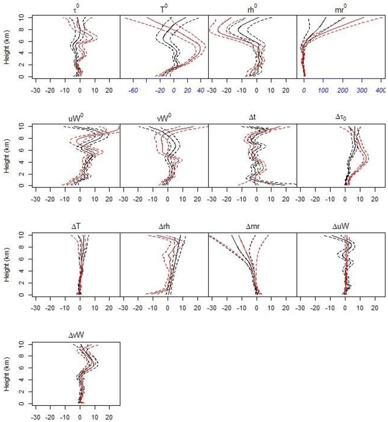
Fig. 11 Initial (black) and heteroskedasticity-adjusted (red) estimated functional coefficients \hat{\nu}_q for the functional variance model (4) of pressure collocation mismatch. Note that the axis in blue ( T^0 and mr^0 ) are on a different scale and that the black and red estimates are not directly comparable
