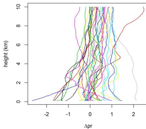
Fig. 4 Collocation mismatch profiles of pressure
