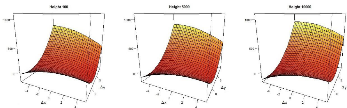
Fig. 10 \delta_{\Delta}(\Delta x, \Delta y, h) for three different values of height
