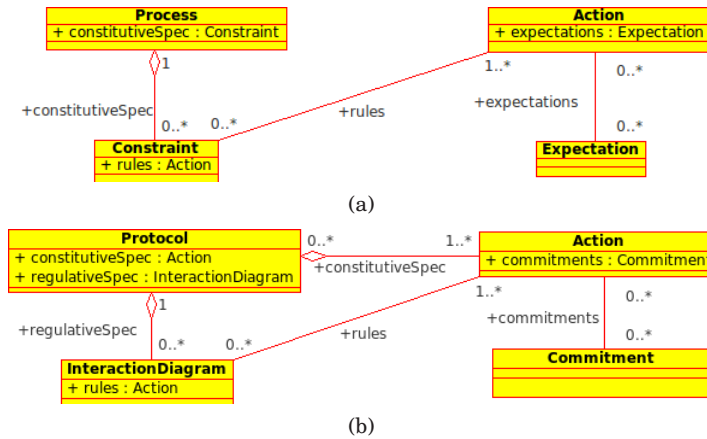
Fig. 2. (a) ConDec model: constitutive specification given by means of constraints on actions, an extension supplies an expectation-based semantics for actions; (b) Fornara and Colombetti's model: regulative specification given by interaction diagrams defined on actions.
