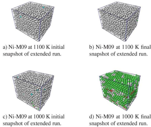
Figure 13 Snapshots of the extended simulations (additional 2 million steps) at 1100 and 1000 K to examine stability of the amorphous phases. At 1100 K, the simulation remained in an amorphous state, while at 1000 K crystallization occurred leaving two fcc slabs with crystalline defects and a grain boundary between them. Green atoms represent local fcc environments, red corresponds to hcp, cyan is icosahedral, and grey is ‘other’ (no recognized structure).
