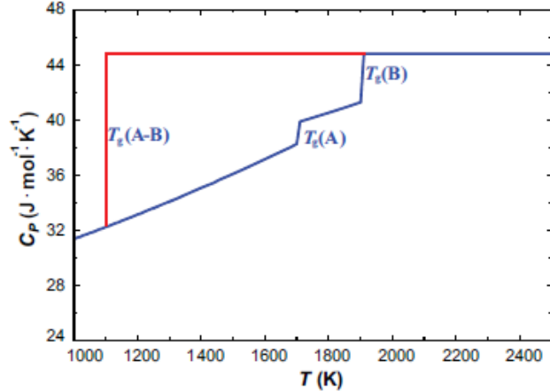
Figure 6 Heat capacity of A–B liquid at X(B) = 0.5 . C_p of the liquid phase is estimated from the pure liquid components by the Neumann–Kopp rule. The solid lines are calculated assuming that the heat capacities of the pure liquid components drop at their glass transition temperatures. The dashed lines are calculated assuming that the heat capacities of the pure liquid components remain constant and drop only at T_g of the solution.
