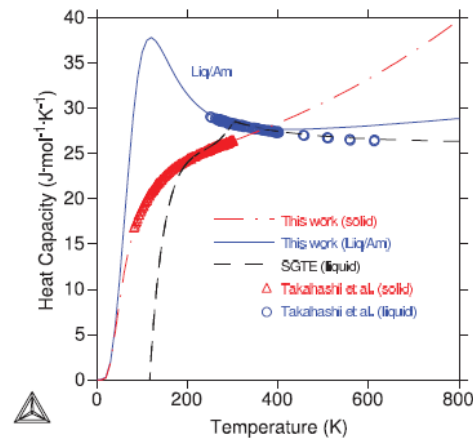
Figure 8 The heat capacity of solid and liquid Ga. Three parameters were optimized for the liquid to fit the melting temperature, the heat of melting and the heat capacity of the liquid at the melting temperature. The entropy term G_m^d was fixed to the value of the entropy of melting as given by SGTE. The result is compared to experimental data [11].
