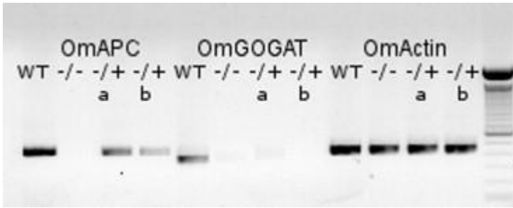
Fig. 5. Semiquantitative RT-PCR on RNA extracted from mycelia grown on media supplemented with \text{NaNO}_3 as nitrogen source for 30 days, on OmAPC15 , OmGOGAT and OmActin genes. WT = wild type strain; -/- = OmGOGAT/OmApc15 -disrupted strain; -/+a and -/+b OmAPC15 -recomplemented strains.
