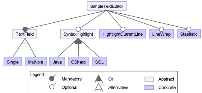
Figure 30: Feature diagram of the STE
