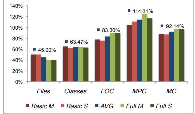
Figure 31: Results of the quantitative evaluation. Each bar represents the DELTAJ 1.5 measurement relatively to the ECLIPSE RCP measurement.
