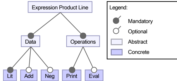
Figure 1: Feature model for Expression Product Line
