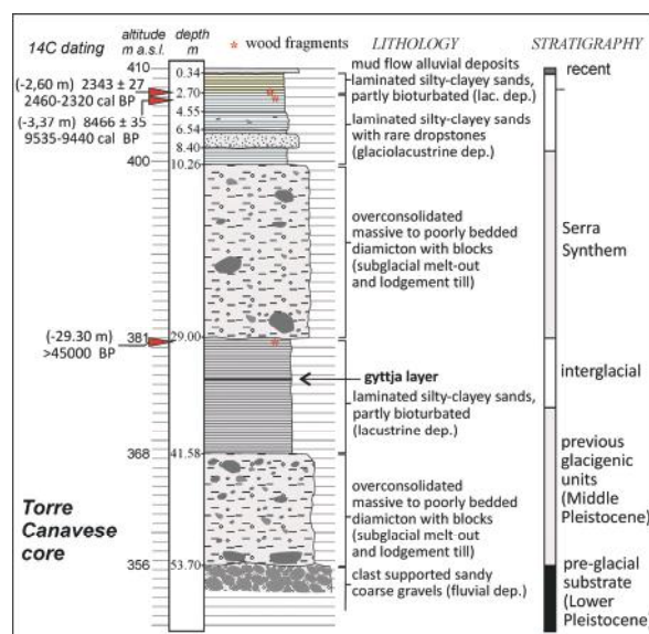
Fig. 13 - Lithological data and preliminary stratigraphical interpretation of the Torre Canavese log in the Ivrea morainic end system (2 in Fig. 5). Radiocarbon ages were calibrated using OxCal v3.10. Calibrated dates are with 95.4% probability.
