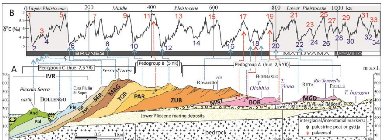
Fig. 17 - (A) Geological cross-section of the IMA lateral north-eastern sector, where all the stratigraphical units have been recognized. Profile trace is shown in Fig. 14 (trace a). Interglacial or interglacial markers are indicated with asterisks: 1) Bosa Palaeosol; 2) Sorgente Solfurea peat layer; 3) Comunità palaeosol; 4) Gianetto gyttja layer. (B) The glacial sequence is tentatively related to the subsequent Pleistocene glaciations. The correlation is made with the global isotopic curve from Lisieki & Raymo (2005), which is a synthesis of 57 benthic marine oxygen isotope records.
