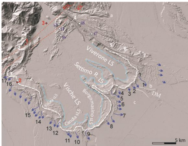
Fig. 4 - The main glacial lobe (LS) and sub-lobe (sLS) systems are marked on the DTM of the IMA by dashed white line (during Internal Serra stadial) and blue dashed line (during Piverone stadial). Other minor LS are reported (white numbers): Riccardi (1), Alice Superiore (2), Strambinello (3), Pré Lake (4), Magnano (5), Santo Sudario (6), Salussola (7). The locations of the drill cores used for stratigraphic reconstruction are mapped with red symbols (1: Alice Superiore; 2: Torre Canavese; 3: Montalto Dora). The erratic boulders dated with cosmogenic nuclide dating method are pointed out by white squares (i7 and i8 on the External Serra crest; i1, i3 and i6 in the Ivrea Hills). Black numbers indicate the spillway/glaciofluvial fan systems forming the proximal sandur. From east to west they are the spillways of Cavaglià (1), Dora Morta (2), Passo d'Avenco (3), Sapel da Bras (4), Bocca d'Arbaro (5), Suc (6), San Maurizio (7), Moncrivello (8), Mazzè (9), Valle della Motta (10), the three opening of Caluso (11), Candia (12), Barone Canavese (13), Montalenghe (14), outer Taglio Grosso (15), Ronchi (16) and Pramonicco (17). Letters indicates elements explained in the text.
