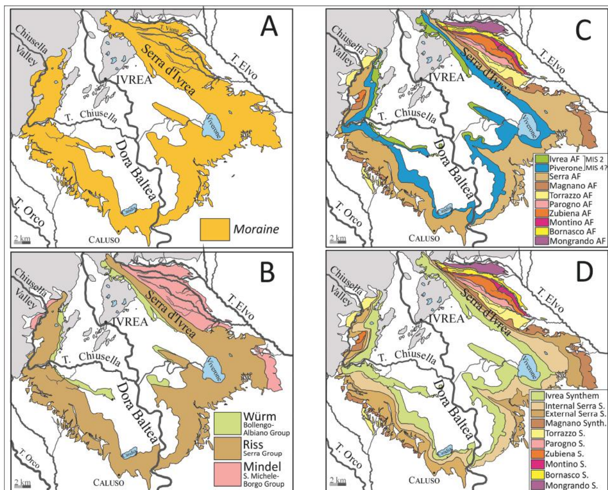
Fig. 6 - The stratigraphic mapping of the IMA according to different models on glaciations. (A) Only one long glaciation model (second part of XIX century). (B) Four glaciations separated by long interglacials according to Penck & Brückner (1894-1980ss). (C) Many glaciations separated by short interglacials (end of 20 th century-Present). (D) Nine glaciations of the present work.
