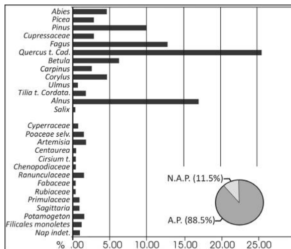
Fig. 16 -The Alice Superiore core palynological spectrum, derived from a unique sample from a peaty clayey layer at 52 m depth, with good preservation and high pollen concentrations (>111 000 grains/g) (redrawn from Arobba et al., 1997).
