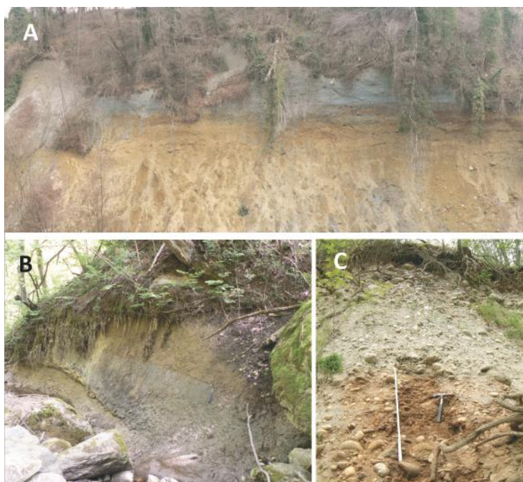
Fig. 9 - Photos of interglacial markers in the IMA. (A) Rio Rudo palaeosol well-exposed in the right side of the Rio Rudo incision, separating the Serra subglacial till (below) from the Ivrea subglacial melt-out till (above). (B) Glaciotectionized Cascina Gianetto gyttja layer separating the Parogno subglacial till (below) from the Torrazzo glacial sequence (above). (C) Glaciofluvial gravel of the Piverone subsystem (LGM) resting above a weathered glaciofluvial gravel of the pedogroup B (Torrazzo or Parogno synthems) (abandoned quarry near Mazzé).
