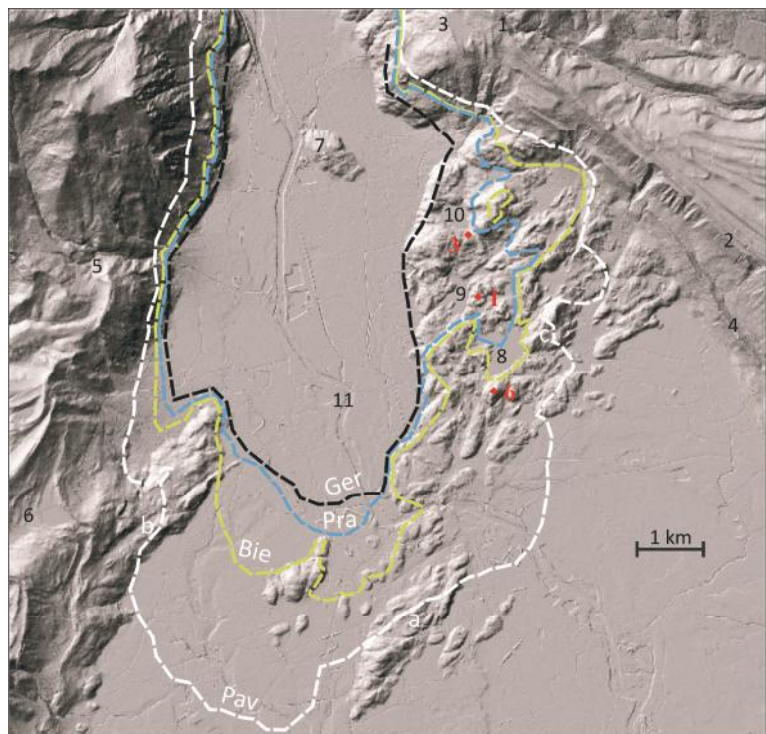
Fig. 11 - Reconstruction of the halts of the Dora Baltea Glacier front during the LGM stadials in the Ivrea Hills area: Pavone (Pav), Bienca (Bie), Prà San Pietro (Pra) and Germano (Ger) stadials. Locations of samples (Ivrea1, 3 and 6) for ^{10}\text{Be} exposure dating are indicated by red numbers and symbols. 1) Starting point of the Serra d'Ivrea; 2) Serra d'Ivrea moraine; 3) starting point of the Piccola Serra at Andrate 4) Piccola Serra moraine; 5) starting point of the right lateral moraine at Brozzo; 6) Alice Superiore LS and Lake; 7) Monte Buono monadnock; 8) Sirio Lake; 9) Pistono Lake; 10) Black Lake; 11) Dora Baltea River (on DTM, courtesy of Piedmont Region).
