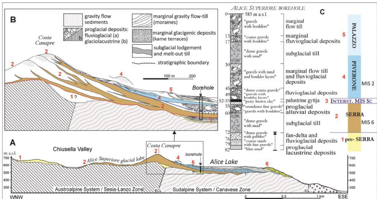
Fig. 14 - Stratigraphical reconstruction of the IMA northwestern sector (cross section trace b in Fig. 14), based on the attribution of the Alice peat layer to the MIS 5c interstadial (from Gianotti et al., 2008, mod.). According to this, the Serra Synthem (MIS 6) must correspond to the lower 12 m thick subglacial till body. The upper 13 m thick subglacial till body has to include the the Piverone and Palazzo subsynthems (MIS 2) and is correlatable with the slightly more external succession of moraines and kame terraces. The coarse gravels lying above the interstadial layer are referred to as anaglacial proglacial (45-49 m) and marginal deposits (30-45 m) of the Piverone Subsynchronism. The similar coarse gravels lying at the top of the succession should be cataglacial proglacial (13-17 m) and stadial marginal deposits (0-13 m) of the Palazzo Subsynchronism. In the detailed profile (B) only the subglacial tills are colored. The dotted lines indicate the basal surfaces of the LGM (blue line) and of the MIS 6 (red line) glacial successions.
