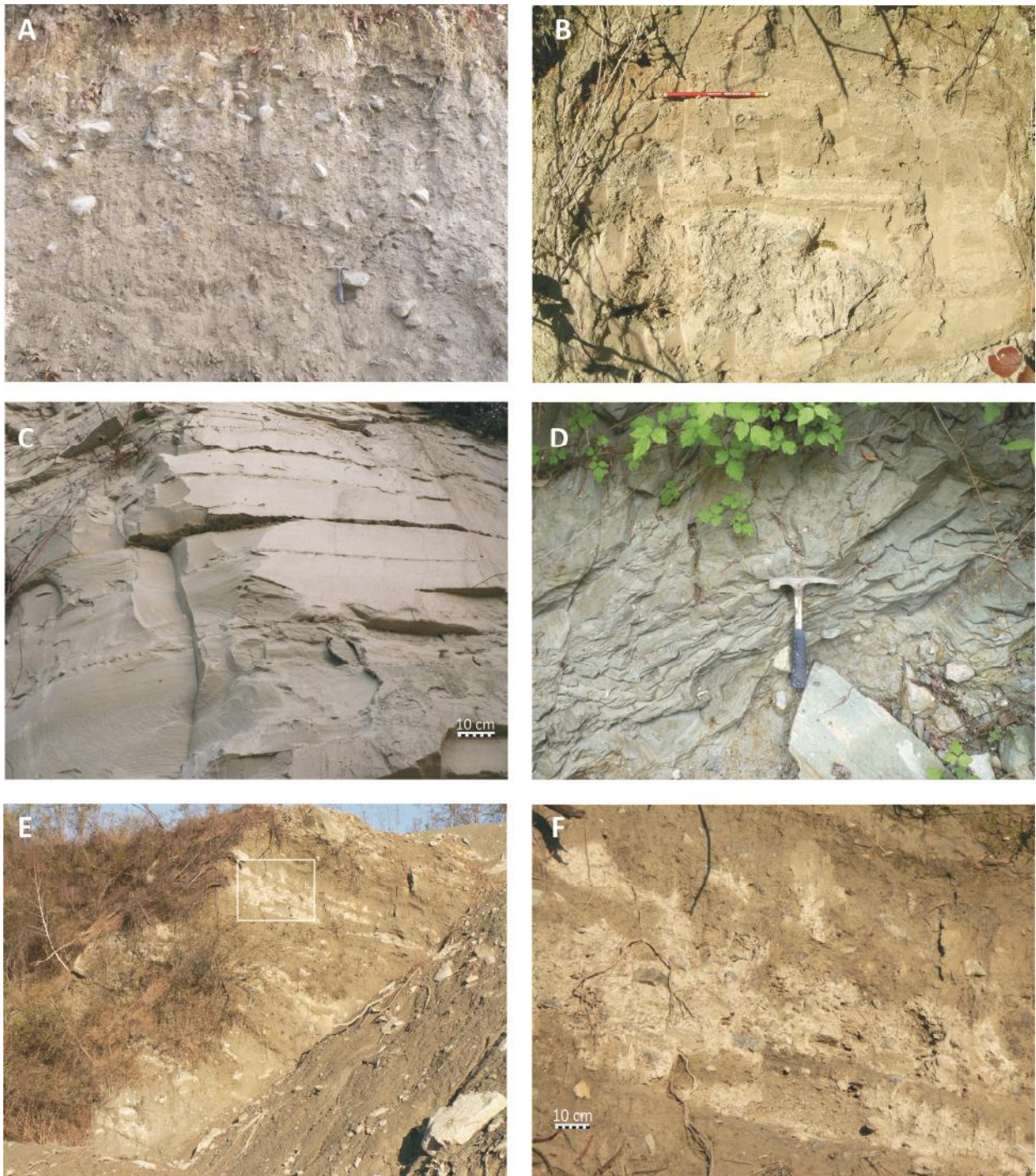
Fig. 10 - Different facies of glacial deposits cropping out in the IMA. (A) Lodgement till of the Internal Serra subsynthem (Palazzo). (B) Submarginal melt-out till forming the M. Bicocca frontal moraine, referred to the External Serra subsynthem (Mazzé). (C) Proglacial glaciolacustrine bottomset deposits of the Piverone subsynthem, made of parallel-laminated sandy silt (Dora Baltea R. left side, Cascine Francia, SE of Vische). (D) Slices of proglacial glaciolacustrine clayey silt resulted from subglacial thrusting during the Torrazzo glacial expansion (Riale di Parogno creek near Cascina Gianetto, Magnano). (E-F) Submarginal melt-out till forming the Parella frontal moraine truncated by the Chiusella R. incision (Andrate subsynthem, South of Parella). Note the up-glacier dipping stratified sediments conforming to the inner slope of the moraine (E). The white box indicates the detail of the diamicton shown in F.
