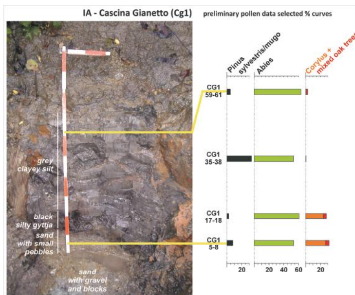
Fig. 15 - The lacustrine layer of Cascina Gianetto and its preliminary pollen data selected % curves (from Gianotti & Pini, 2011).
