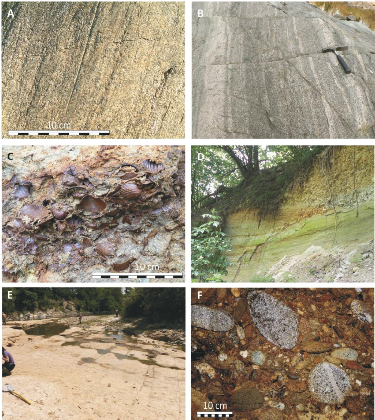
Fig. 3 - The various lithotypes that constitute the IMA substrate. (A) Polished and striated basic granulite in the Ivrea Hills (Montalto Dora). (B) Basic granulite of the Ivrea Verbano Zone forming the bedrock cropping out in the Chiusella R. riverbed (Ponte dei Preti, Strambinello). (C) Zanclean fossiliferous marine sediments into the Strambinello LS (Peronetto, South of Parella). (D) Estuarine transitional sand and gravel cropping out into the Borra Grande incision (Peronetto, South of Parella). (E) Fractured villafranchian sandy silt, recently exposed into the Elvo riverbed. (F) Deeply weathered fluvial gravel referred to the pre-glacial Dora Baltea fan (Cerrione synthem), cropping out in the Valle Sorda riverbed (west of Cerrione).
