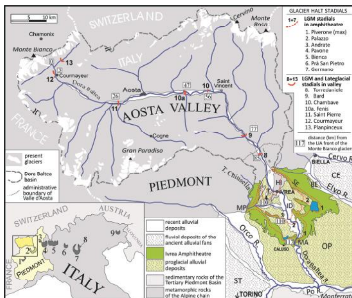
Fig. 1 - Geomorphological sketch map of the Dora Baltea basin, with the 3400 km 2 wide mountain basin nearly corresponding to Valle d'Aosta region and the IMA at the outlet of the valley (from Gianotti et al, 2008, mod.). The present glaciers of the basin are shown. The bedrock crops out in the IMA inner sector in the granulite Ivrea Hills (HI) and in the outer western sector in the Monti Pelati peridotite reliefs (MP). The Serra d'Ivrea moraine (SE), the inner depression (ID) and the outer outwash plain (OP) are pointed out. The Dora Baltea River flows out of the IMA through the Mazzé gorge (MA). At the northeastern edge the Bessa roman gold mines extend (BE). The Stura di Lanzo (ST) and Cervo (CE) fan complexes spread laterally to the IMA. LGM to Lateglacial stadials in Colli d'Ivrea area and in the valley are shown. Main morainic amphitheatres of Italian Alps (box at the bottom left): 1 Rivoli-Avigliana (Susa Valley); 2 Ivrea (Dora Baltea Valley); 3 Orta (Strona Valley); 4 Verbano (Ossola+Ticino valleys); 5 Lario (Valtellina and Como Lake); 6 Iseo (Camonica Valley); 7 Garda (Adige-Sarca valleys); 8 Rivoli Veronese ("Lagarina" Valley); 9 Tagliamento (Tagliamento Valley).
