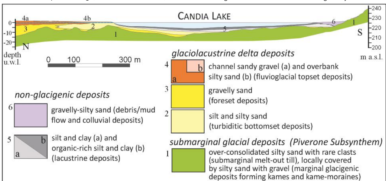
Fig. 12 - Geological cross-section of the Candia Lake area derived from geophysical surveys (from Colombero et al., 2014, modified). The articulated shape of the deepest resistivity boundary suggests the presence of buried kame-moraines of submarginal till (1). The extent of fine glaciolacustrine deposits (2 and 3) both under the lake and the plain suggests the wider extent of a former lake. The current Candia Lake is the relict of a wider ice-dammed lake, not completely filled up by deltaic deposits coming from the retreating Dora Baltea glacier. The filling up of the lake suddenly slowed down owing to the complete retreat of the glacier (5a) and continued so far (5b) by a moderate colluvial and alluvial supply from the southern side of the basin (6).
