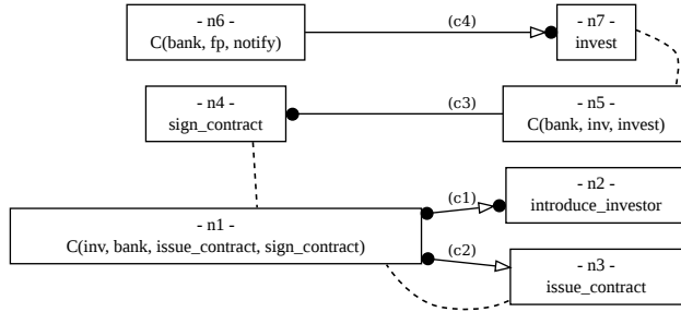
Fig. 7 Graphical representation of the 2CL constraints from the sale protocol. Dashed lines highlight relationships between events/facts and commitments.
