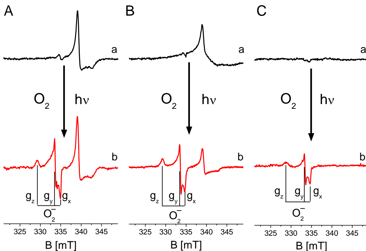
Figure 5. EPR spectra of A: CZ05_SGI; B) CZ05_SGN; C) CZ05_HYD . a) background and b) spectra obtained with irradiation under oxygen atmosphere. All b) spectra have been recorded at 77K after irradiation with visible light ( \lambda > 420\text{nm} ) in \text{O}_2 atmosphere.
