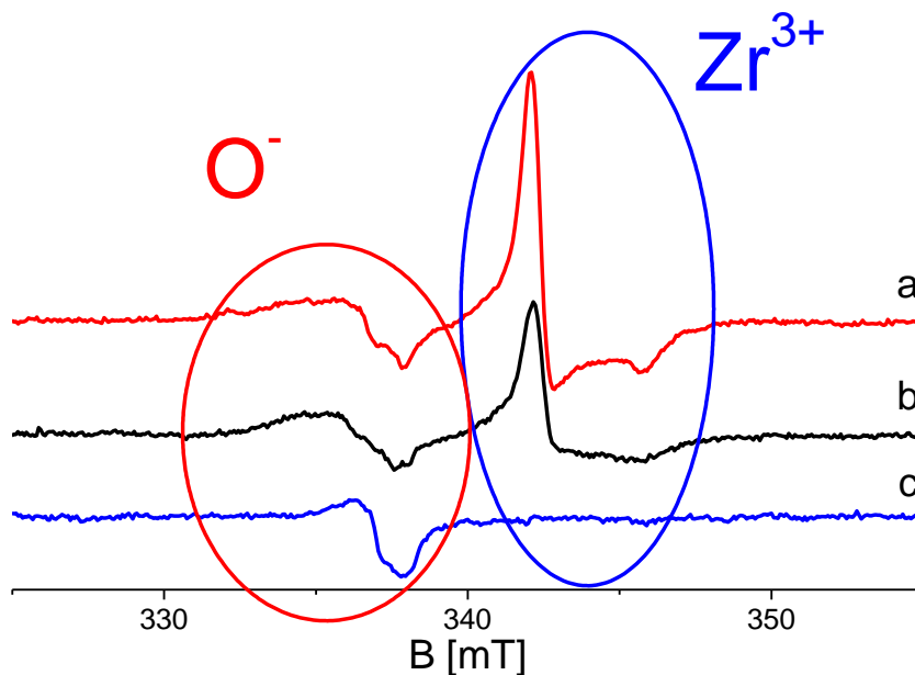
Figure 4. EPR spectra evidencing the formation of trapped charge carriers upon irradiation under vacuum ( \lambda > 420 nm) of a) CZ05_SGI, b) CZ05_SGN, c) CZ05_HYD.
