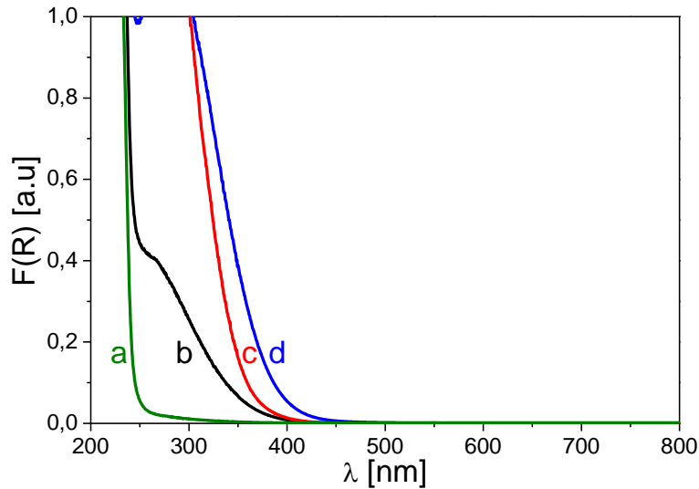
Figure 2. Absorbance spectra of ZrO 2 (a), CZ05_SGI (b), CZ05_SGN (c) and CZ05_HYD (d).
