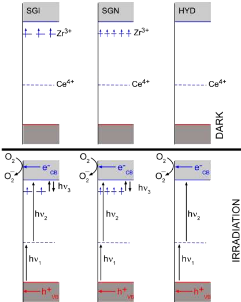
Figure 6. Schematic illustration of the electronic structure of the three materials in dark (upper part) and under irradiation (lower part). The figure evidences the documented formation of holes, electrons and superoxide species using photons with energy far lower than the band gap.
