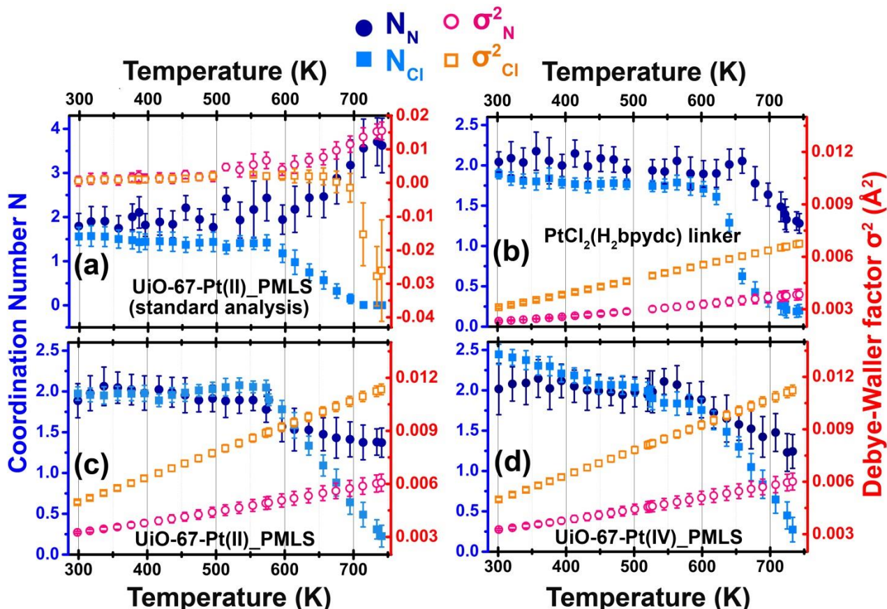
Figure 7. Part (a): standard analysis of the operando TPR-EXAFS series of spectra collected on UiO-67-Pt(II)_PMLS. Each EXAFS spectrum has been analyzed as single datum, independently from the other spectra. In the (300-600) K range, although relatively high error bars and some non-physical oscillations, reported values are meaningful. In the 600-750 K range reported values correspond to good mathematical fits of the experimental data, that has however no physical meaning. Parts (b)-(d): final refinement of the operando TPR-EXAFS experiments on PtCl 2 (H 2 bpydc) linker and on UiO-67-Pt(II)_PMLS, UiO-67-Pt(II)_OPS, and UiO-67-Pt(IV)_PMLS, respectively. Data referring to the Pt–N and Pt–Cl bonds are reported as blue and cyan full-symbols and refer to the left ordinate axes. Corresponding Debye-Waller factors are reported as pink and orange open symbols and refer to the right ordinate axes. The latter were refined with a parametric approach using the Einstein model, see Eq. (1). The Einstein temperatures \Theta_E obtained for both Pt–N and Pt–Cl bonds from this study are reported in Table 2. All experiments were performed adopting a temperature gradient of 3 K min -1 . A selection of the experimental data used in these analyses is reported in Figure 6.
