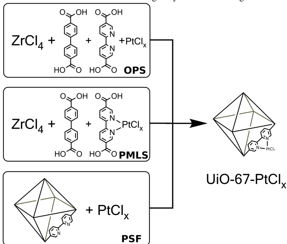
Figure 2. Scheme of the three different synthesis procedures adopted to obtain the final product UiO-67-bpy-PtCl x ( x = 2 or 4 ), part (d). Part (a): mixing in one-pot ZrCl_4 and PtCl_x precursor salts react with biphenyl and bipyridine linkers (OPS). Part (b): mixing biphenyl and PtCl_x(H_2bpydc) ( x = 2 or 4 ) pre-functionalized bipyridine linkers (PMLS). Part (c): reacting pre-made UiO-67-bpy MOF with precursor PtCl_x salt.
