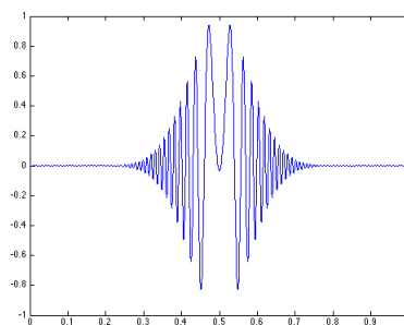
FIGURE 2. Initial values. The right one is numerically supported in [0.25, 0.75]
