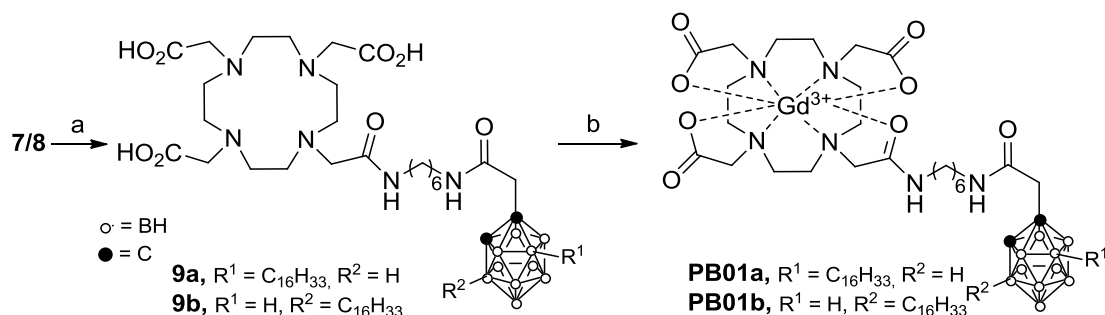
Scheme 3 Synthesis of Gd 3+ -C-[(COOH) 3 DOTAMA-C 6 ]-acetamido-C'-H-4-(hexadecyl)-ortho-carborane ( PB01a ) and Gd 3+ -C-[(COOH) 3 DOTAMA-C 6 ]-acetamido-C'-H-9-(hexadecyl)-ortho-carborane ( PB01b ). Reaction conditions and yields: a) CF 3 COOH, CH 2 Cl 2 , r. t., (>99% for both 9a and 9b ); or H 2 , Pd/C, EtOH, CH 2 Cl 2 , rt (>99% for both 9a and 9b ); b) GdCl 3 , H 2 O (>99% for both PB01a and PB01b ).
