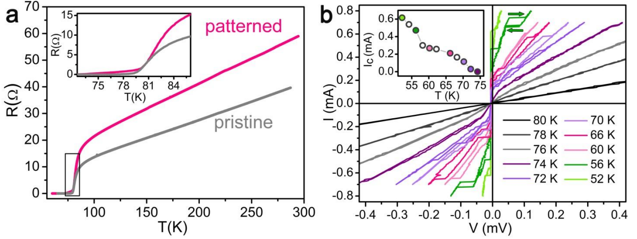
Figure 2. a) Comparison of the resistance versus temperature behaviour measured in the four-probe configuration between pristine and patterned conditions. The inset represents a magnification of the superconducting transition region. b) I-V characteristics of a patterned device measured at constant temperatures between 52 and 80 K. The green arrows exemplify the typical hysteretic pattern in the case of T = 56 K. The inset shows the temperature behaviour of the corresponding critical current values I_c . Void circles refer to curves that have not been shown in the main panel for clarity.
