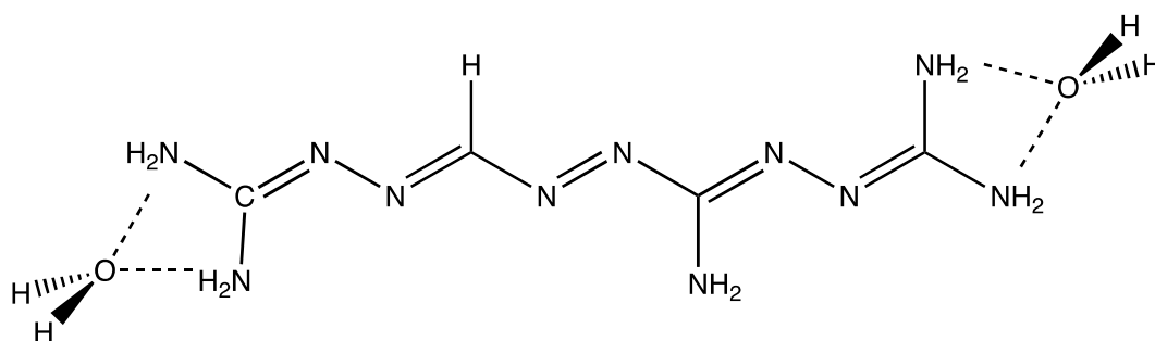
Scheme 4. Sketch of the 3 •2H 2 O moiety present in the asymmetric unit of the hydrated P&G phase.
