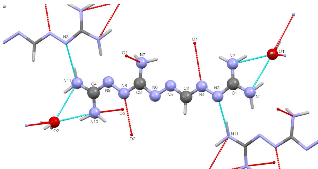
Figure 1: Ball and stick representation of the asymmetric unit of 3 •2H 2 O highlighting the network of H-bonds (HB). Both water molecules are involved in four HB (O1 and O2 behaving both as HB-acceptors toward the guanidine ends, and as HB-donors toward N4, N7 and N8, N10, respectively); N1 and N2 only act as HB-donors toward O1; N10 acts both as HB-donor and -acceptor toward O2;
