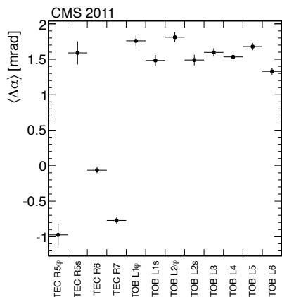
Figure 14: Kink angle \Delta\alpha for double-sensor modules, averaged over layers (L) and rings (R), respectively. Stereo (s) and r\varphi ( \varphi ) modules within the same layer or ring are separated.
