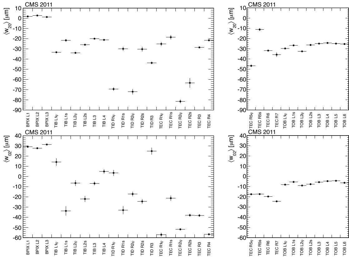
Figure 13: Sensor curvatures along the local u (upper row) and v (lower row) coordinate for single- (left column) and double-sensor (right columns) modules, averaged over layers (L) and rings (R), respectively. Stereo (s) and r\varphi ( \varphi ) modules within a layer or ring are separated.
