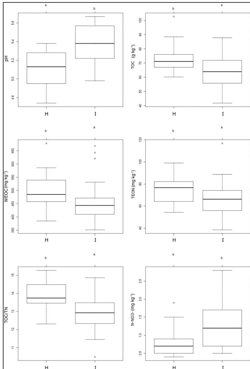
207 208 Fig. 4. Boxplots (n = 60) of pH values, TOC, WEOC, TEON, TOC/TN and \text{N-NO}_3^- content of topsoils in 209 hummock apexes (H) and interhummocks (I). Letters indicate statistically significant differences.
