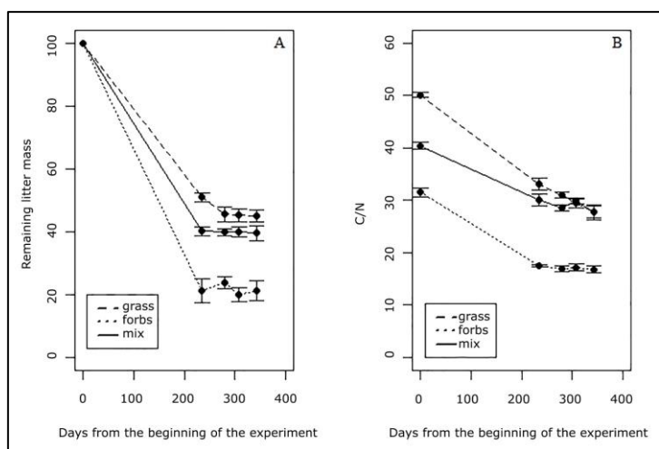
298 Fig. 7. Remaining litter mass (%) (A) and C/N ratio (B) for the three litter types (Grass, Forbs and Mix) during 299 the one year long decomposition experiment.
