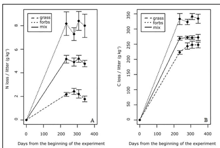
309 Fig. 8. Nitrogen (A) and carbon (B) loss of the three litter types (Grass, Forbs and Mix) during the one year 310 long decomposition experiment.
