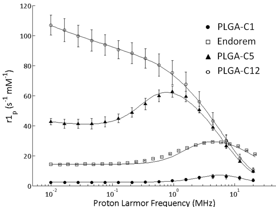
Figure 3. Profiles of 1/T_1 ^1H -NMRD (25°C and pH=7.4) of PLGA-Fe-NPs loaded with the different magnetic nanoparticles: C12 ( \circ ), C5 ( \blacktriangle ), Endorem ( \square ), and C1 ( \bullet ). The solid lines between data
