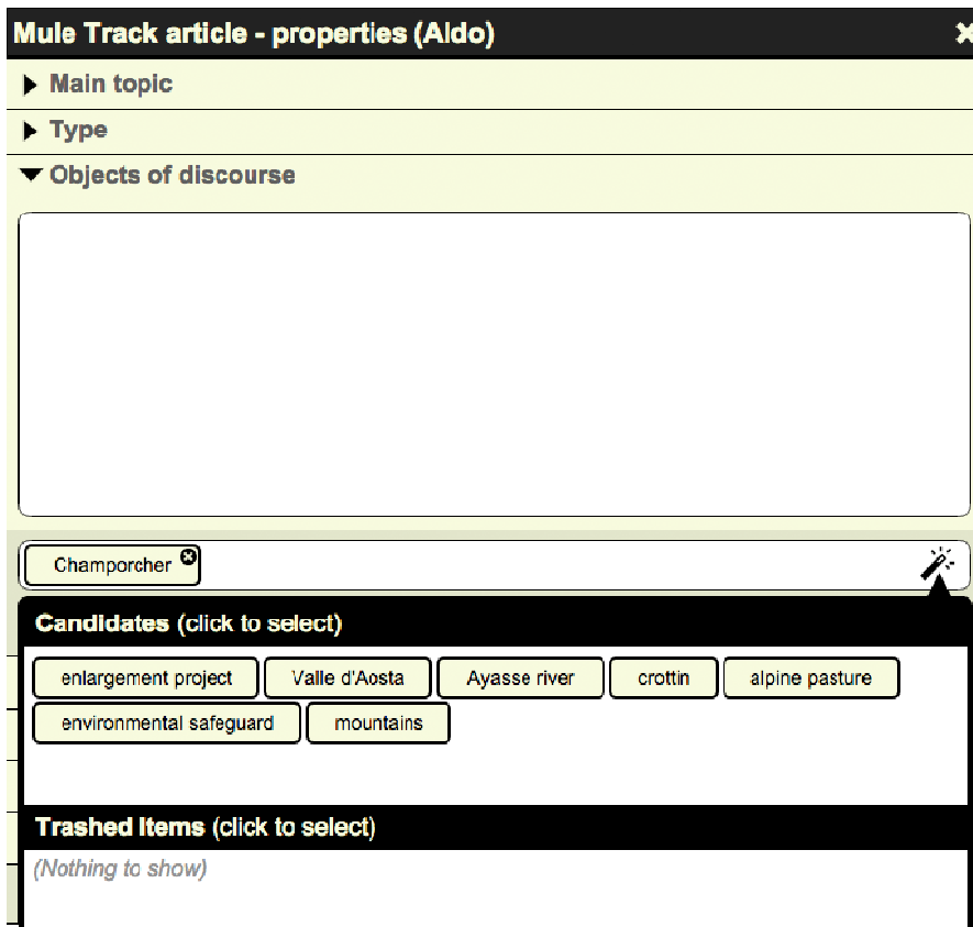
Fig. 3. SemT++ UI displaying semantic annotation of a new table resource
