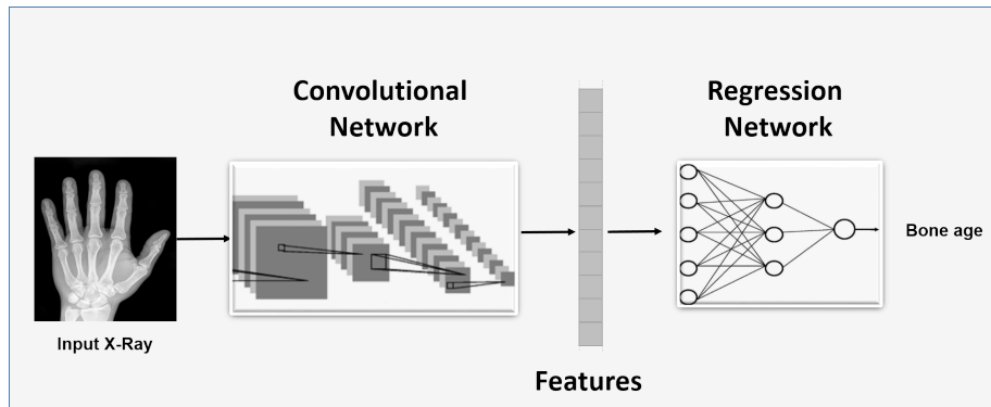
Figure 2: General architecture of deep learning methods for bone age assessment. It consists of a) a convolutional network consisting of an arbitrary number of convolutional layers (that can be derived from pre-trained CNN models or can be designed from scratch) for feature extraction; and b) a regression network consisting of a set of fully connected layers (generally one or two) and a linear scalar output layer providing the bone age estimate.
