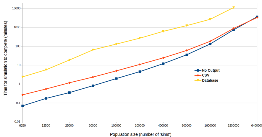
Figure 10: The time taken (in minutes) for simulations of THIM implemented in JAS-mine to complete for a variety of population sizes. The three lines correspond to different data export options, with 'Database' referring to persistence to the output relational database, 'CSV' referring to the export of data to separate comma-separated values files, and 'No Output' referring to the benchmark case where no data is exported. Simulations were executed on the ARCUS-B cluster of the University of Oxford's Advanced Research Computing facility.
