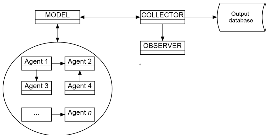
Figure 3: The structure of JAS-mine's Manager classes. The Collector acts as an intermediate layer between the Model class (which controls the model specification such as agents, their interaction and environment) and the Observer (which displays information about the state of the simulation in the Graphical User Interface). The Collector aggregates information about the model objects (agents), and calculates any statistics needed either by the Model's objects (agents) themselves or for the Observer. The Collector can export the data to the output database or to csv files as required.
