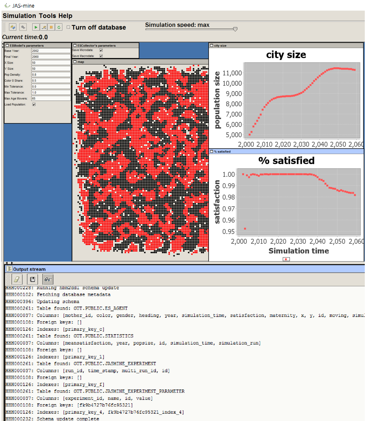
Figure 8: Interactive Mode: screenshot of the JAS-mine graphical user interface showing output from the Extended Schelling demonstration model, available at www.jas-mine.net/demo/extended-schelling .
