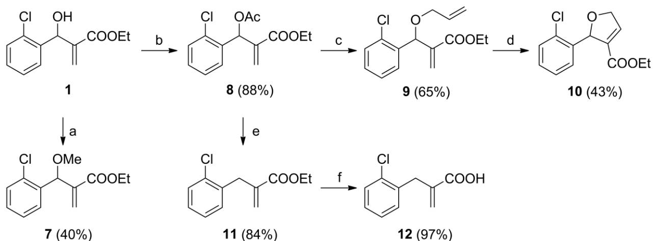
Scheme 2. Synthesis of compounds 7–12
