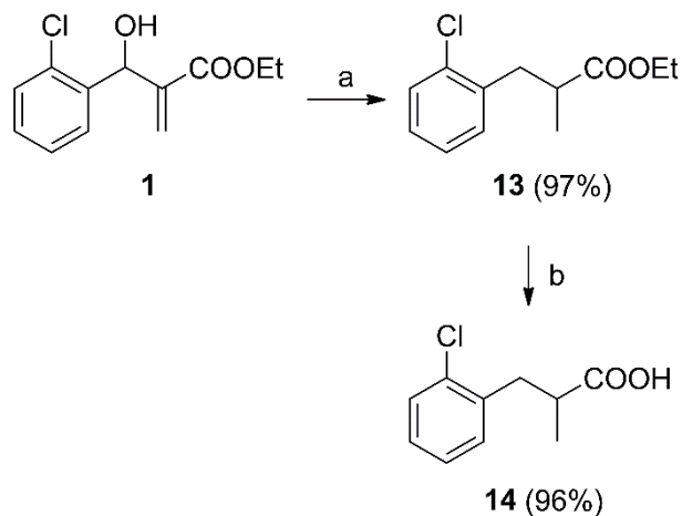
Scheme 3. Synthesis of compounds 13–14
