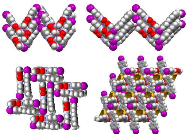
Figure 4. Herring-bone motifs and \pi – \pi stacking in crystalline 3A (top left; only the main image of disorder is shown), 3B (top right, isomorphous with 2 ) and 3solv (bottom left and bottom right); the yellow contour surfaces represent the large pores probably occupied by solvent in non-stoichiometric amount.
