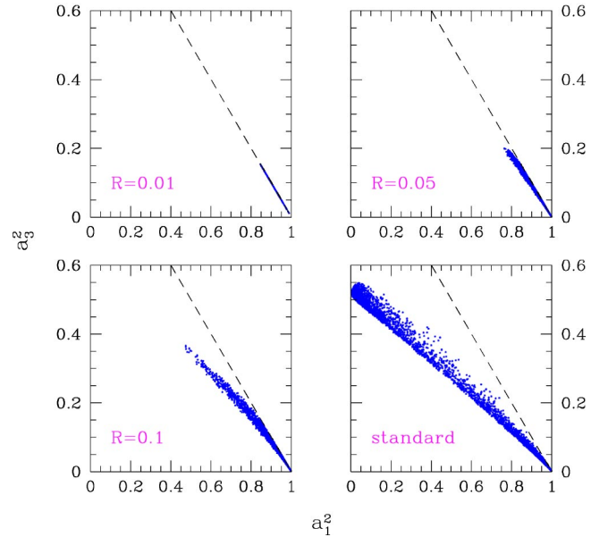
FIG. 4. Scatter plots of the neutralino composition in terms of \tilde{B} ( a_1 ) and of \tilde{H}_1^0 ( a_3 ) for R=0.01, 0.05, 0.1 and for the standard value R=5/3 \tan^2 \theta_W \approx 0.5 . The dashed lines denote the line where a_1^2 + a_3^2 = 1 .
