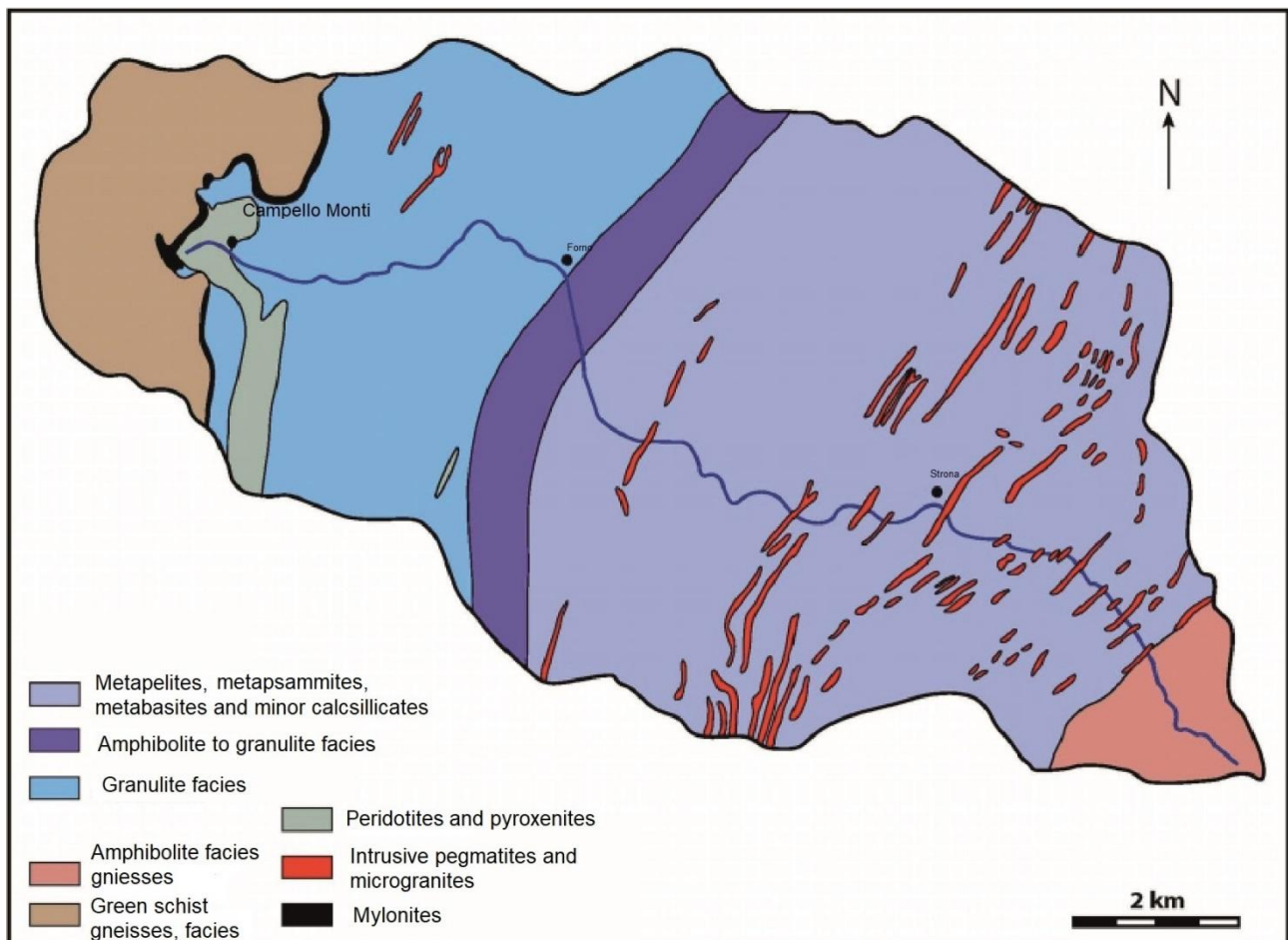
Fig. 2. Simplified lithological map of Val Strona of Omegna (modified from Bea and Montero, 1999).
