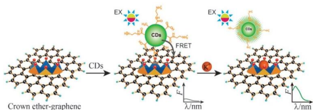
Fig. 7 Schematic illustration of the FRET model based on Cd dots-graphene and the mechanism of \text{K}^+ determination. Reprinted with permission from Ref. 37 Copyright (2012) The Royal Society of Chemistry.
