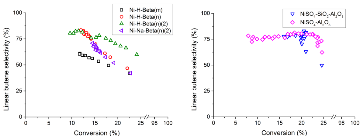
Figure 9: Linear-C 4 - selectivity versus conversion for zeolite (left) and NiSO 4 -containing (right) catalysts. Reference reaction conditions: 29 bar total pressure where P ethene = 25.1 bar and P inert = 3.9 bar and T = 120 °C
