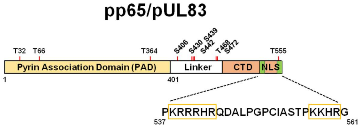
Figure 2 - Schematic representation of the viral tegument protein pp65. Sequence revealed a conserved N-terminal Pyrin Association Domain (PAD) (yellow box), a divergent linker region (white box), and a conserved C terminus (CTD, ~90 residues) (brown box), indicating a bipartite structure. The conserved NLS motifs (KRRRHR/KKHR) are also shown. Numbers located above each diagram represent phosphorylation sites. Numbers located below each diagram represent phosphorylation sites.
