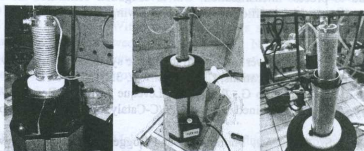
Figure 2: Sonochemical flow-mesoreactors
