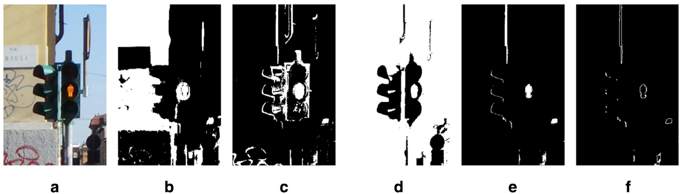
Fig. 12. Extraction of candidates AOUs. (a) Portion of original image, (b) filter on H, (c) filter on S, (d) filter on V, (e) conjunction of filter results, (f) extracted contours.
