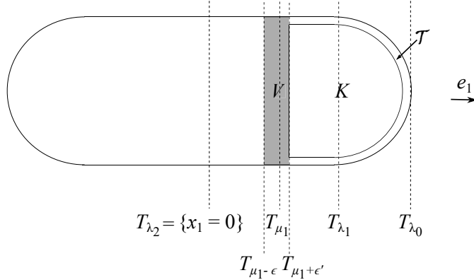
FIGURE 2. Qualitative representation of the domain \Omega , its optimal cap \Sigma_{\mu_1} in the assumption by contradiction, and its subsets K , \mathcal{T} and V defined in the proof.
