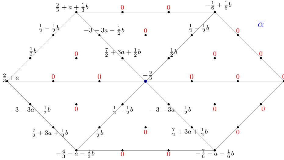
Figure 9: Mask \bar{\alpha} for the construction based on \mathcal{D}_3 .
