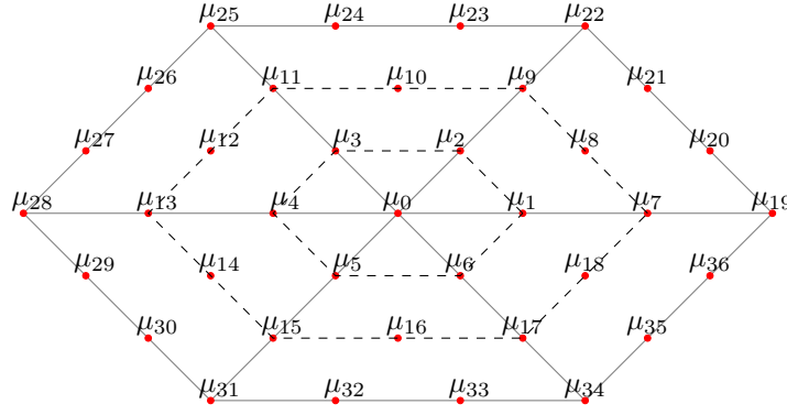
Figure 8: Ordering a general sequence \mu representing f_{i,j}(\mathcal{D}_3) , or any of the masks \bar{\alpha} , \bar{\beta} , \bar{\gamma} and \bar{\omega}_k , 0 \leq k \leq 5 .
