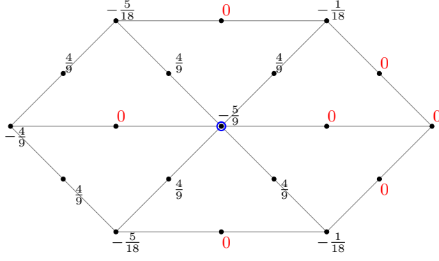
Figure 5: Mask \alpha for the evaluation of the BB-coefficient associated with the point v_{i,j} .
