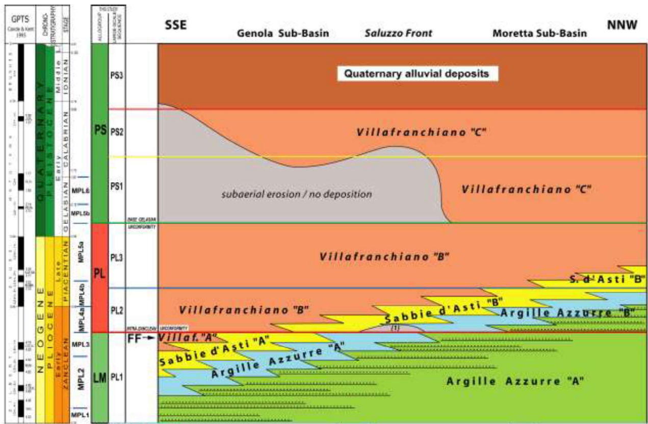
(1) condensed sedimentation or erosion on intrabasin submarine structural high
