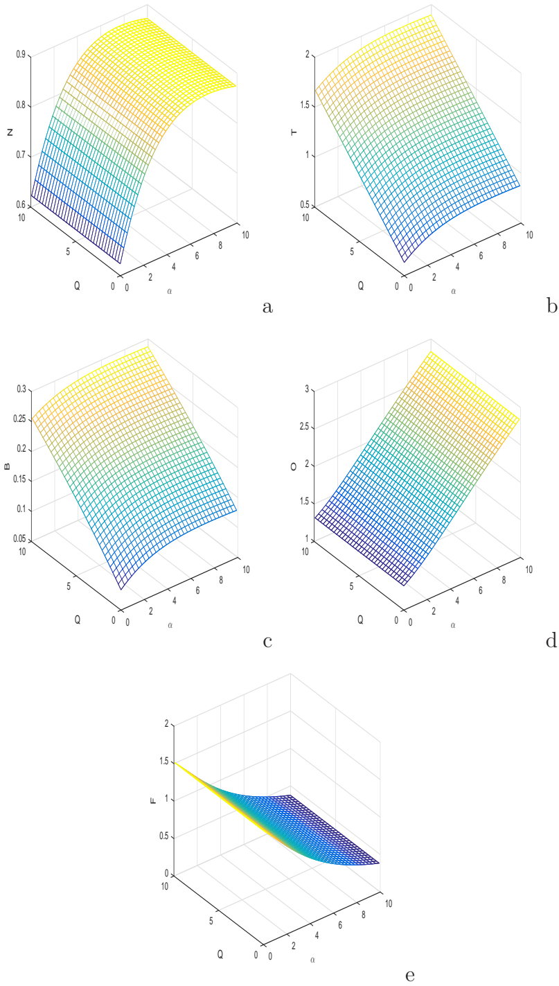
Fig. 6. Variation in (a) human population, (b) organic pollutants, (c) bacteria, (d) DO and (e) fish populations with respect to \alpha and Q . Rest of the parameter values are the same as in the Table 1.
