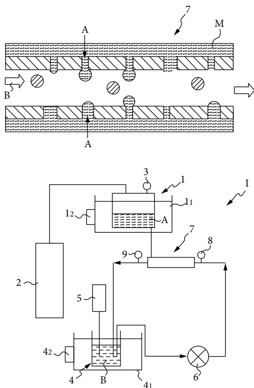
FIGURE 4: Scheme of the membrane contactor module. A (lipid phase), B (aqueous phase), M (porous membrane), 1 (pressurized vessel containing the lipid phase), 1 1 (thermostated bath), 1 2 (thermostat), 2 (nitrogen bottle), 3 (manometer), 4 (vessel containing the aqueous phase), 4 1 (thermostated bath), 4 2 (thermostat), 5 (stirrer), 6 (pump), 7 (tangential flow filtration unit), and 8-9 (manometer) [35].
