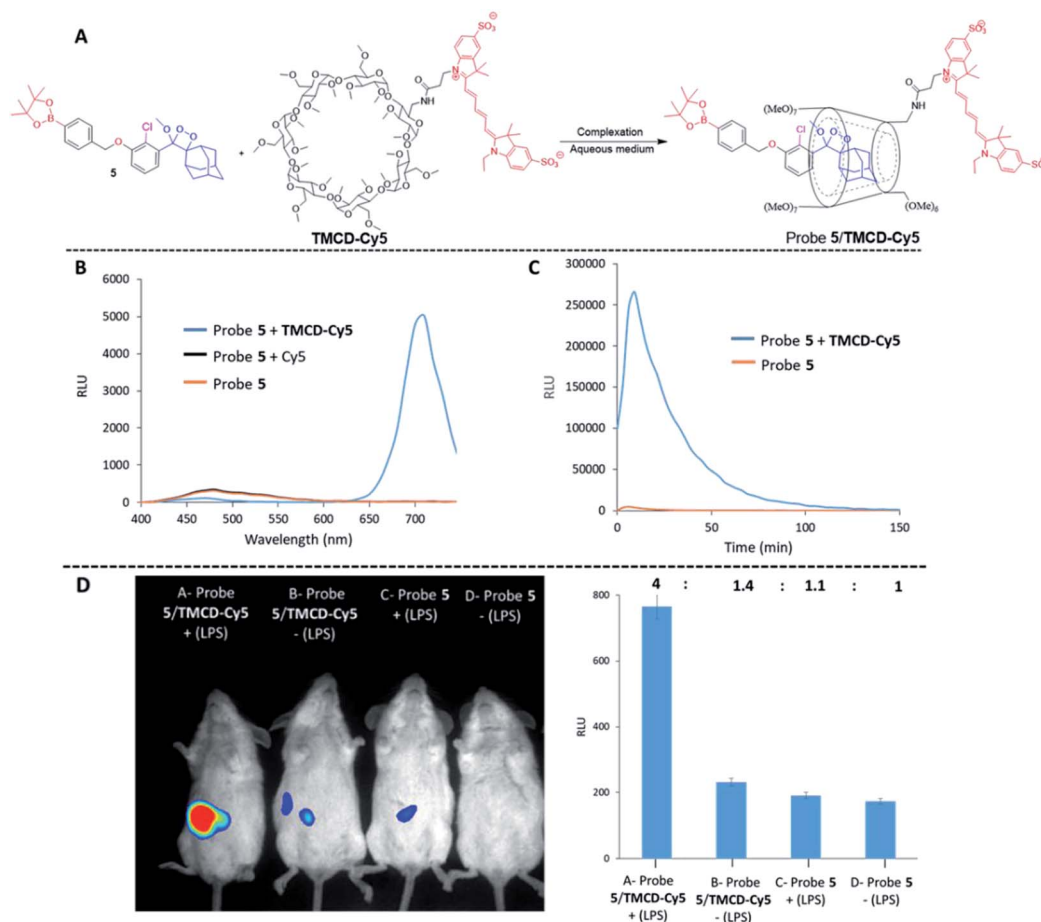
Fig. 8 (A) Chemical structures of probe 5 and TMCD-Cy5. (B) Chemiluminescence spectra and (C) kinetic profiles of probe 5 [100 \mu M] and TMCD-Cy5 [300 \mu M] in PBS, pH 7.4 (1% DMSO). (D) (Left) representative in vivo images of endogenous hydrogen peroxide in the peritoneal cavity of mice during an LPS-induced inflammatory response using probe 5 and TMCD-Cy5. The images of mice were recorded on a BioSpace Lab PhotonIMAGER. For the mice in group A, 1 mL of 0.1 mg mL -1 LPS was injected into the peritoneal cavity, followed 4 h later by an i.p. injection of probe 5 [100 \mu M] and TMCD-Cy5 [300 \mu M] in 100 \mu L PBS, pH 7.4. For group B, 1 mL of PBS, pH 7.4 was injected i.p., followed 4 h later by an i.p. injection of probe 5 [100 \mu M] and TMCD-Cy5 [300 \mu M] in 100 \mu L PBS, pH 7.4. For group C, 1 mL of 0.1 mg mL -1 LPS was injected i.p., followed 4 h later by an i.p. injection of probe 5 [100 \mu M] in 100 \mu L PBS, pH 7.4. For group D, 1 mL of PBS, pH 7.4 was injected i.p., followed 4 h later by an i.p. injection of probe 5 [100 \mu M] in 100 \mu L PBS, pH 7.4. (Right) quantification of signal intensities measured from each group of mice.
