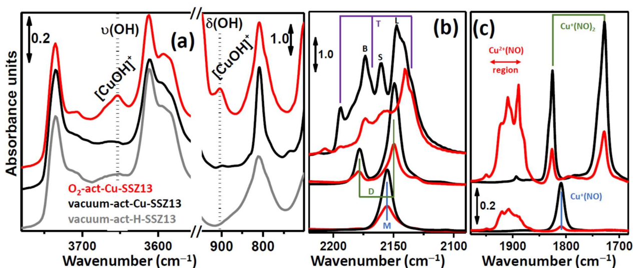
Fig. 3. Low temperature ( \sim 100 \text{ K} ) IR spectra of \text{O}_2 -activated (red) and vacuum-activated (black) Cu-SSZ-13 zeolite ( \text{Si/Al} = 13.1 and \text{Cu/Al} = 0.444 ). Part (a): effect of activation at 400 \text{ }^\circ\text{C} in the \nu(\text{OH}) and \delta(\text{OH}) stretching regions, left and right parts, respectively. For comparison, also the spectrum of the vacuum-activated H-SSZ-13 material (gray) is reported. The \text{O}_2 -activated zeolites presents the fingerprint bands of [\text{CuOH}]^+ species at 3655 and 905 \text{ cm}^{-1} . Part (b): IR spectra of CO adsorption at low, intermediate and high P_{\text{CO}} , bottom, middle and top curves respectively, approximately corresponding to the saturation of mono- (M band), di- (D doublet) and tri-carbonyl (T triplet) complexes. At the highest P_{\text{CO}} , also the bands of CO adsorbed on Brønsted (B), silanols (S) and the band of liquid-like CO are present after both activation. Part c: IR spectra of NO adsorption at low and high P_{\text{NO}} , bottom and top curves respectively, approximately corresponding to the saturation of mono- and di-nitrosyl complexes on Cu(I) sites. In all parts some spectra have been vertically shifted for clarity. Unpublished figure reporting spectra previously published in Ref. 53 for part (a) and in Ref. 65 for parts (b) and (c).
