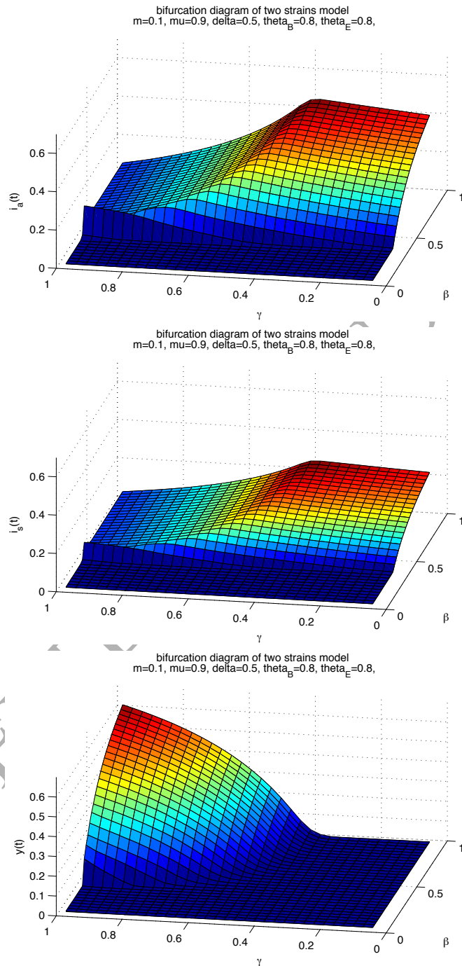
Figure A.6: Trend of the three populations, i_a(t) , i_s(t) and y(t) as functions of \beta and \gamma , for \delta = 0.5 .
