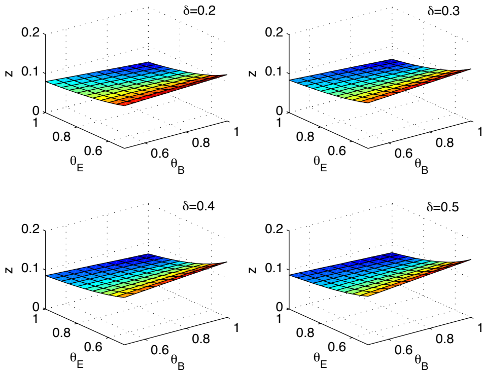
Figure A.4: Surface of equation z = \frac{\mu(\delta + m)}{\mu + \delta} - \theta_B m - \hat{H} as function of \theta_B and \theta_E , for m = 0.1 , \mu = 0.9 and several values of \delta .
