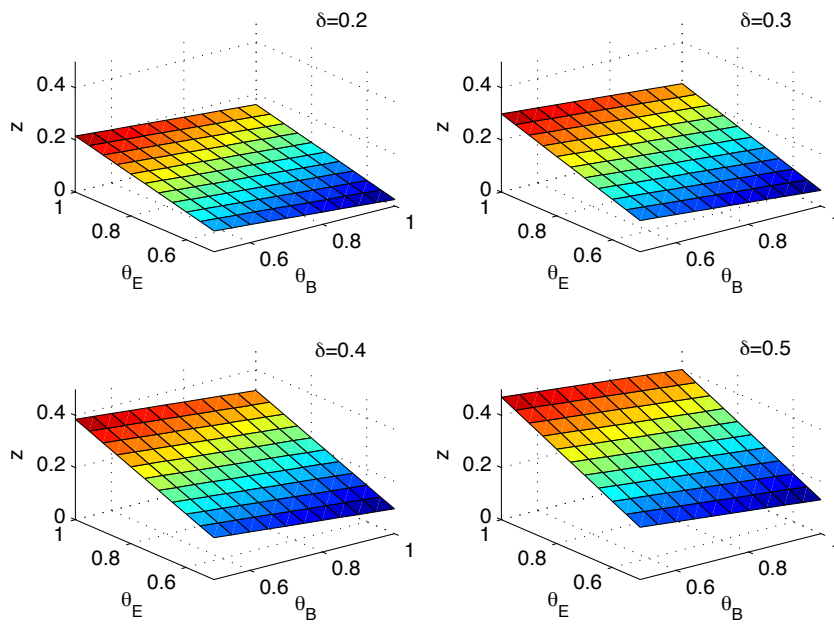
Figure A.3: Surface of equation z = \mu\theta_E(\delta + m) - m(\mu + \delta) = 0 as function of \theta_B and \theta_E for m = 0.1 , \mu = 0.9 and different values of \delta .
