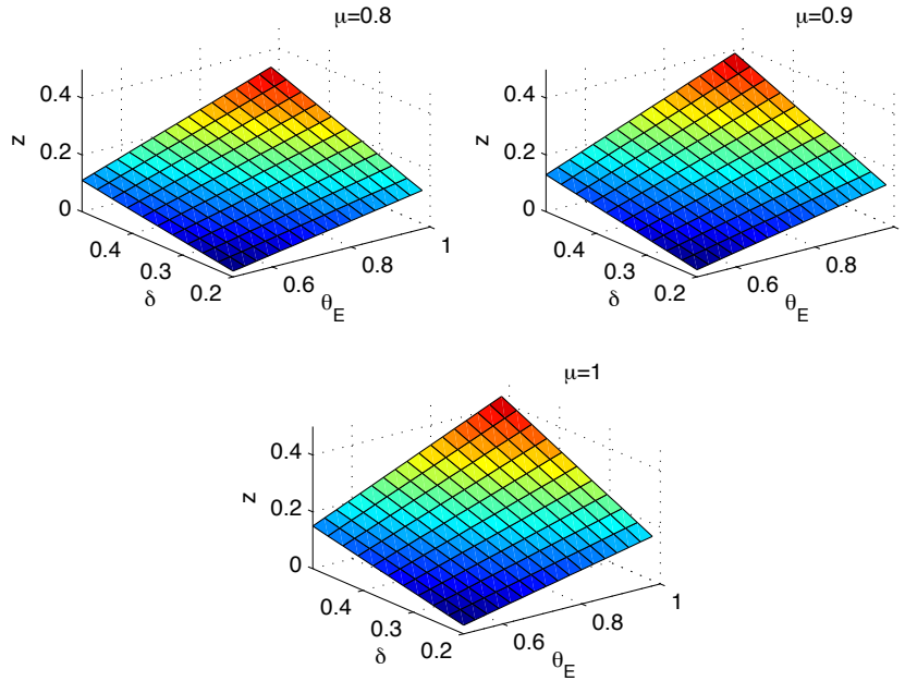
Figure 1: Surface of equation z(\theta_E, \delta) = \mu\theta_E(m + \delta) - m(\mu + \delta) as function of \theta_E and \delta , for m = 0.1 and different values of \mu .
