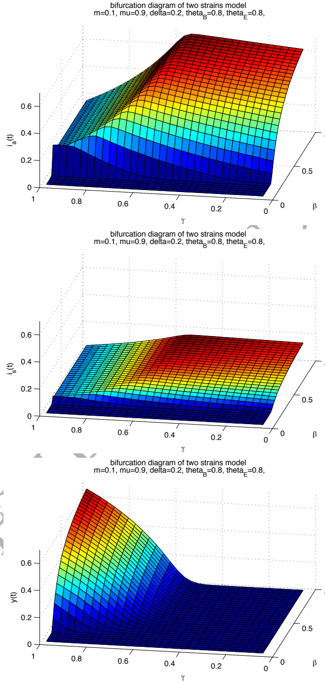
Figure A.5: Trend of the three populations, i_a(t) , i_s(t) and y(t) as functions of \beta and \gamma ,
