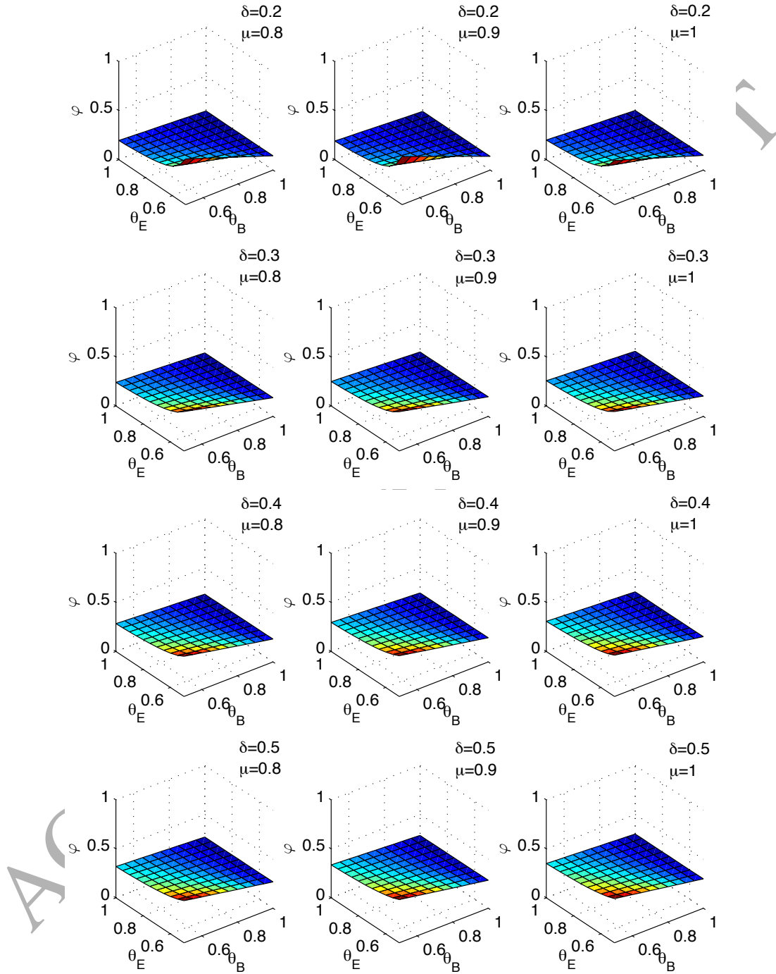
Figure 2: Estimate of the quantity \varphi as a function of \theta_B and \theta_E for m = 0.1 and different values of \delta and \mu .
